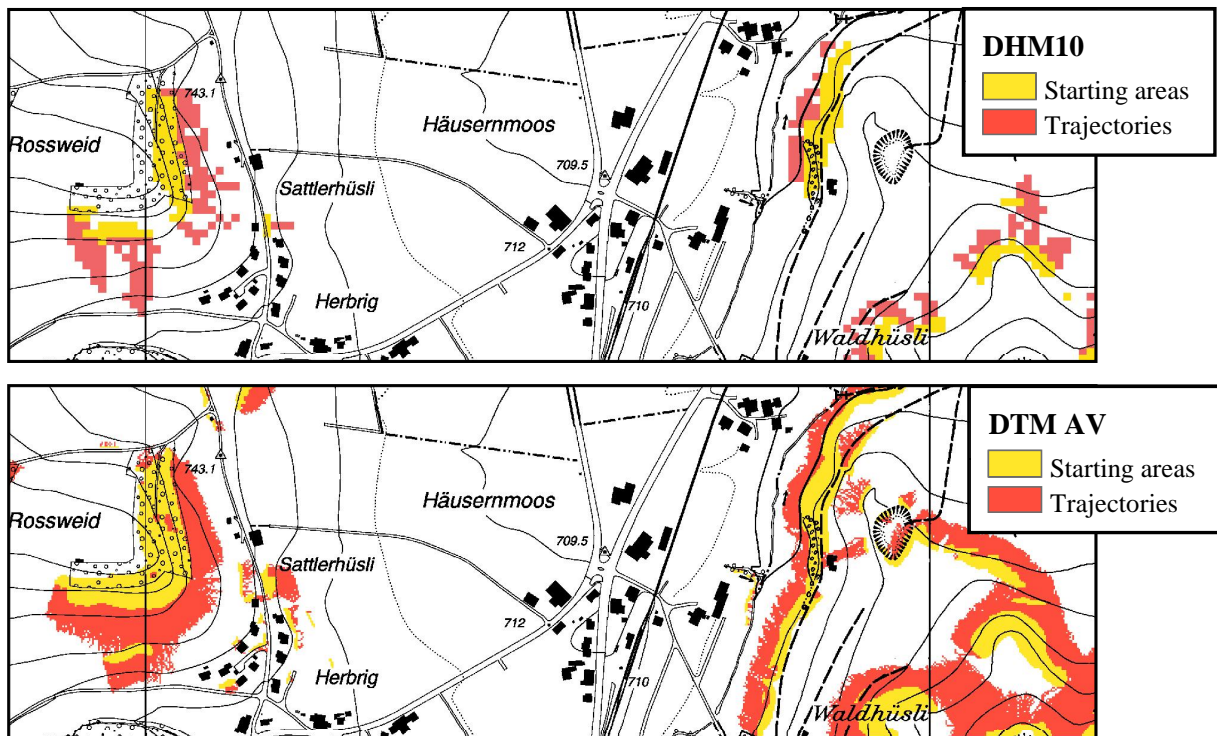
Fig. 1: Comparison of simulation results based on digital elevation model with a resolution of 10 meters (DHM10) above and based on 2 meter resolution DTM-AV below. Both simulations have been done with the same parameters based on different digital elevation models.
